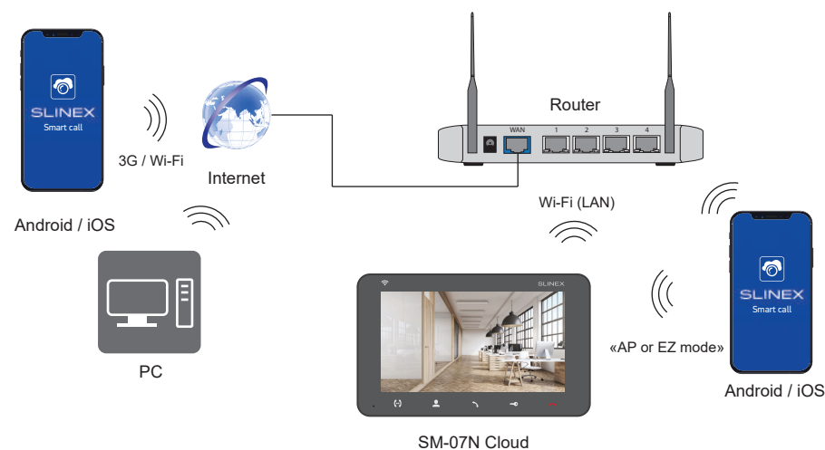
Diagram 2. SM-07N Cloud wireless Wi-Fi network connection.
