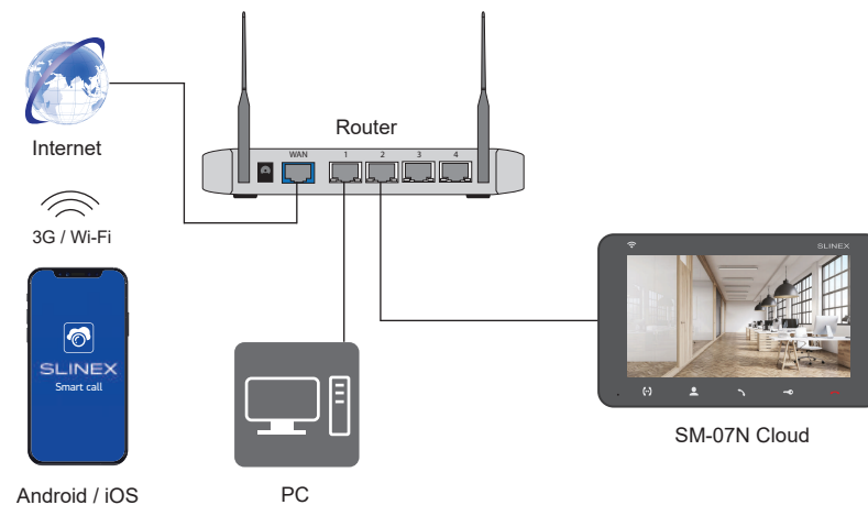
Diagram 1. SM-07N Cloud wired network connection.
